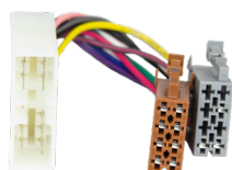
ISO to John Deere 13-Pin
